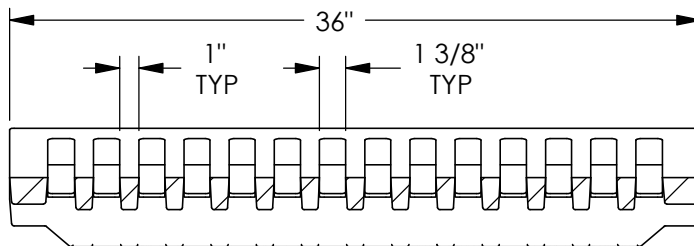
SECTION B-B
